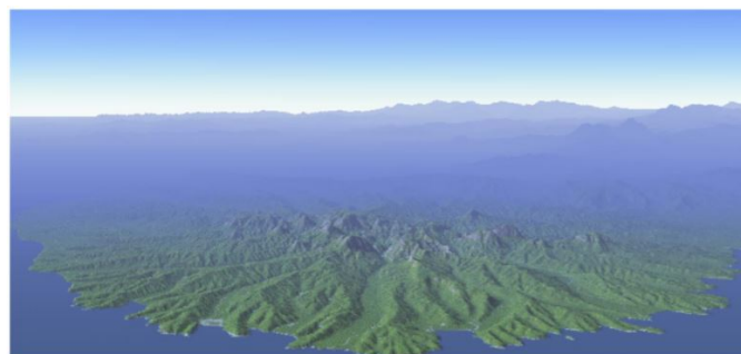
Kunisaki Peninsula viewed from the North. Done by A.G. with digital data courtesy of the Japan National Institute of Geography, on Kashmir 3-D software.
